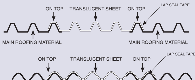
Figure 1 - Laserlite Building Products recommends the use of a strip of 24mm x 5mm Lap Seal Tape
